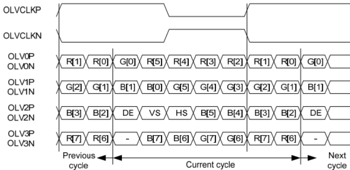
1-port LVDS 8-bit mode with VESA format
