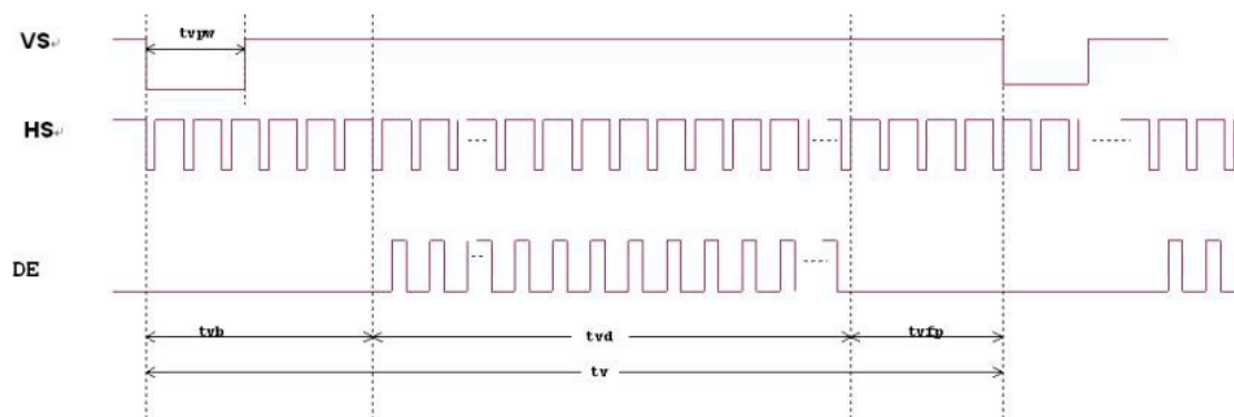
Figure 3. 2 Vertical input timing diagram.
