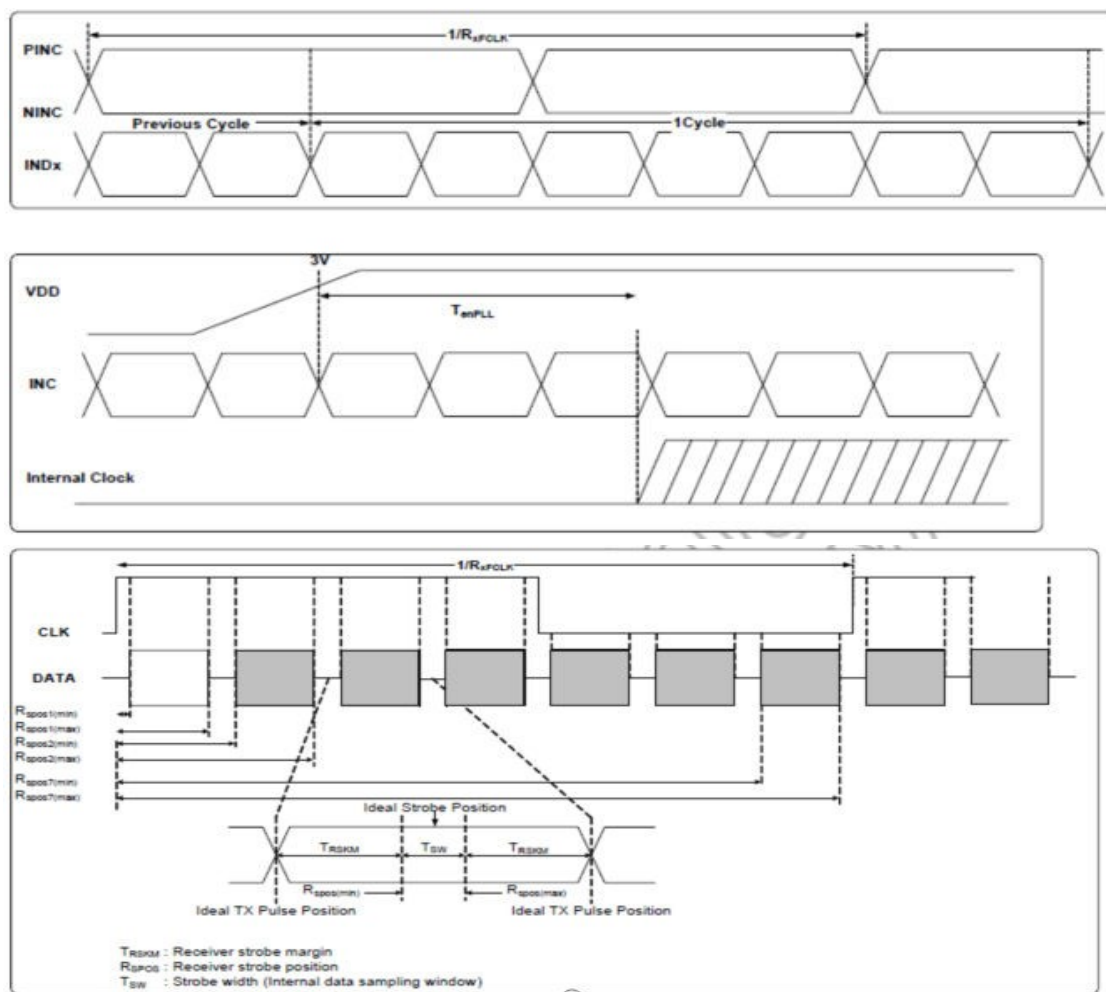
LVDS figure
