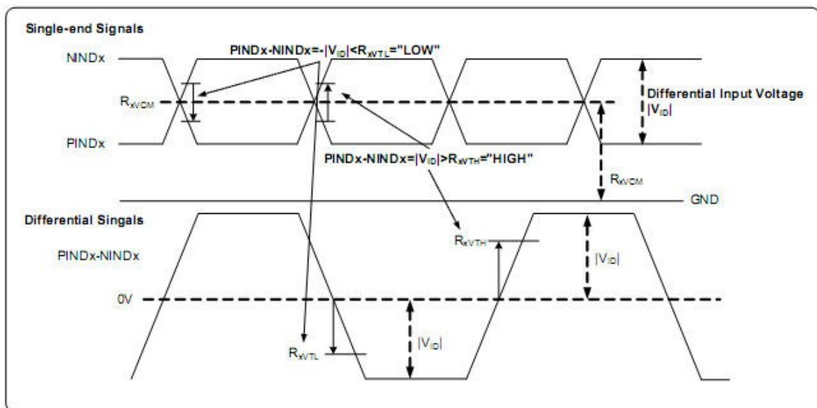
Single-end signals
